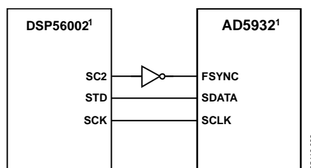
Figure 37. DSP56002 to AD5932 Interface
